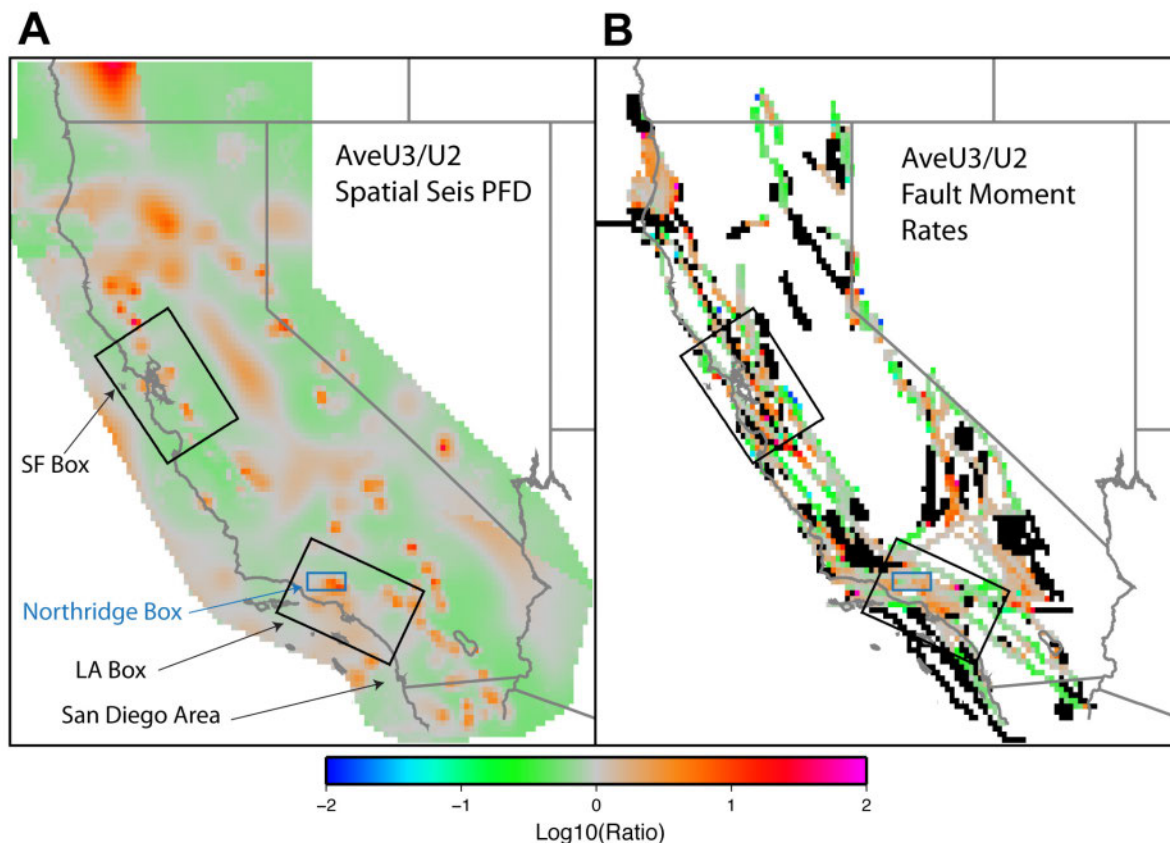
Figure 27. Maps showing ratios of UCERF2 and UCERF3 results. A , Ratio of the average UCERF3 to UCERF2 off-fault spatial seis PFD (equal to 0.5(U2sm+U3sm)/U2sm , where U2sm is the UCERF2 smoothed seismicity map (fig. 14A) and U3sm is the UCERF3 smoothed seismicity map (fig. 14B). This ratio does not include the overall regional rate increase for R_{M \geq 5}^{total} . B , Ratio of branch-averaged, on-fault moment rates between UCERF3 and UCERF2, where infinite values are shown in black (a result of new faults being added where none existed in UCERF2).
