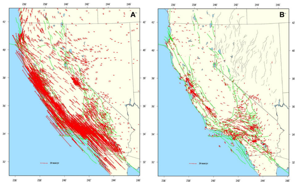
Figure 6. Maps showing GPS velocity vectors for California. A , Distribution of UCERF3 GPS velocity vectors for California, referenced to the North America Plate (from appendix C, this report). B , The residual velocities computed as the difference between observed GPS velocities and those predicted by the UCERF2 Deformation Model 2.1. The velocity scales of the two plots are the same. The residual vectors indicate that UCERF2 generally underestimates the average statewide deformation rate, particularly in the most populated parts of the state.
