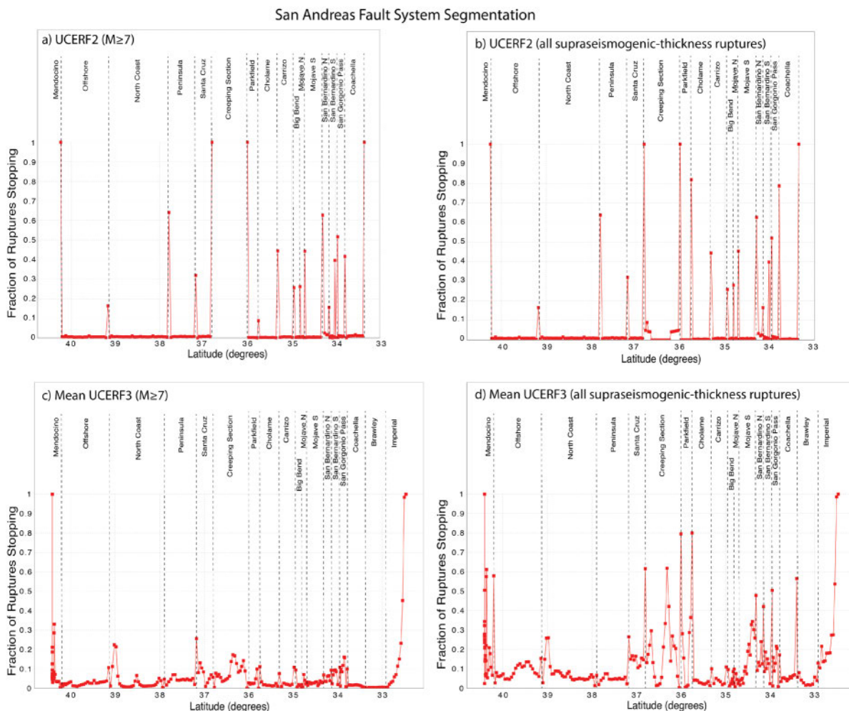
Figure 29. Latitudinal plots showing average model-implied segmentation on the San Andreas Fault system for UCERF2 (top) and UCERF3 (bottom). The right side includes all suprasedimentogenic ruptures, whereas the left side is for only M \geq 7 events. The Brawley and Imperial Faults were not included in UCERF2 (and are therefore not shown for this model). Red points show the rate at which neighboring subsections do not rupture together, normalized by the total rate of ruptures involving those two subsections. Thus, when the red line reaches 1, there is strict segmentation and no ruptures break through that location.
